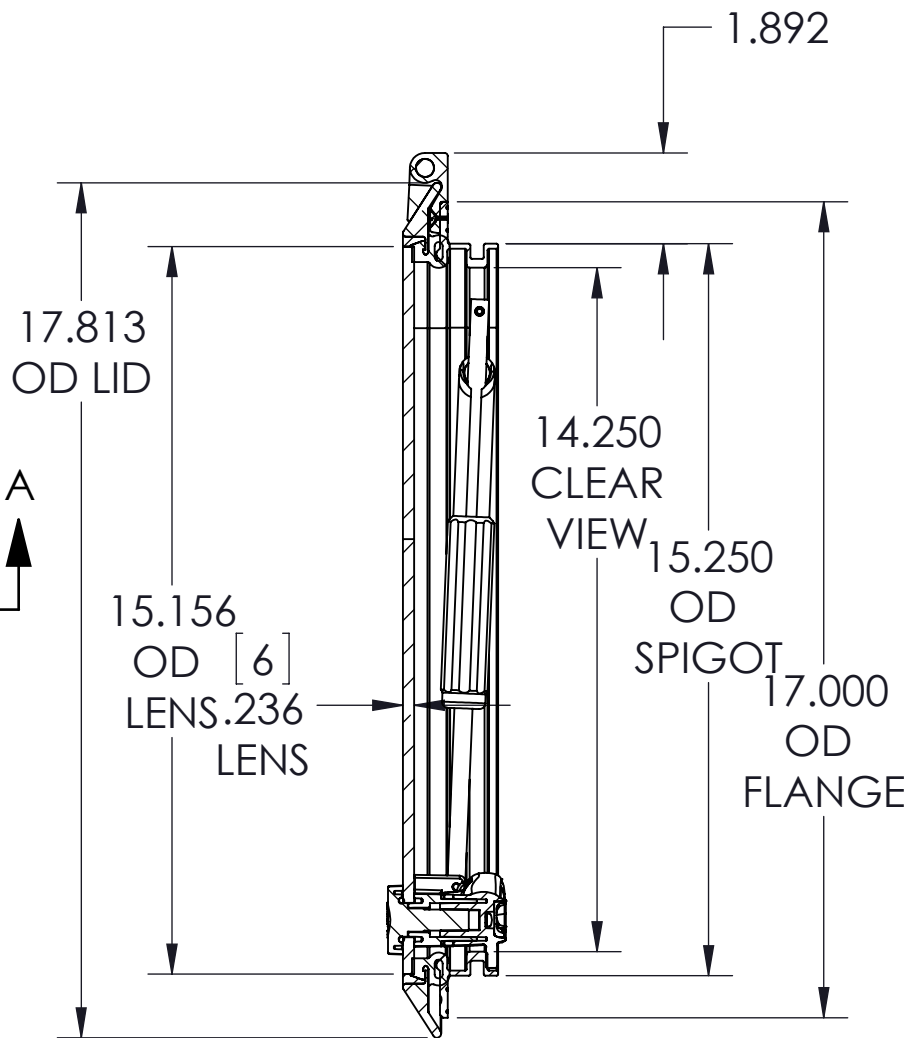
SECTION B-B
